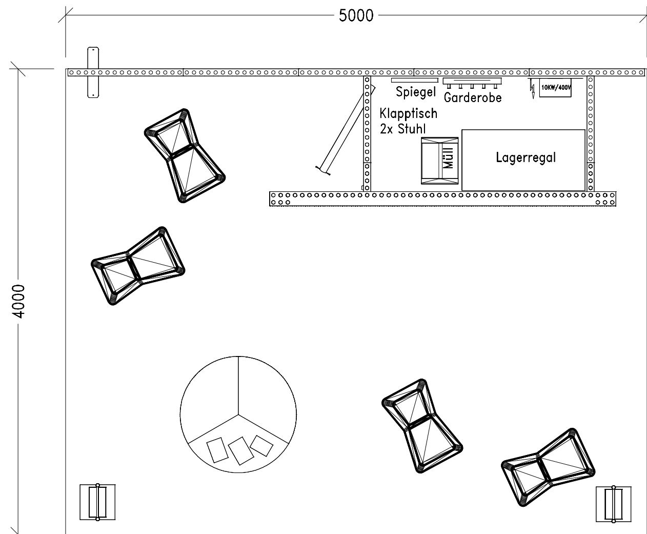
GRUNDRISS FLOOR PLAN
